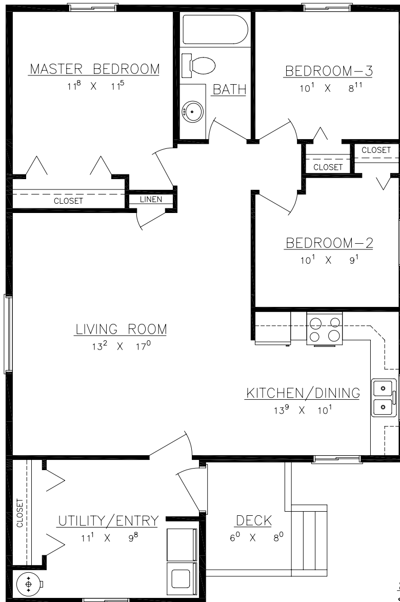
FLOOR PLAN
